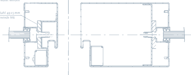
R&M-Sonderzarge
