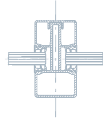
Detail Pfosten
