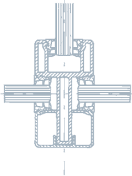
Detail Eckpfosten
